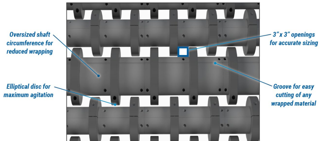
Figure 3: Anti-Wrap Screen Disks (CP Group) 7
