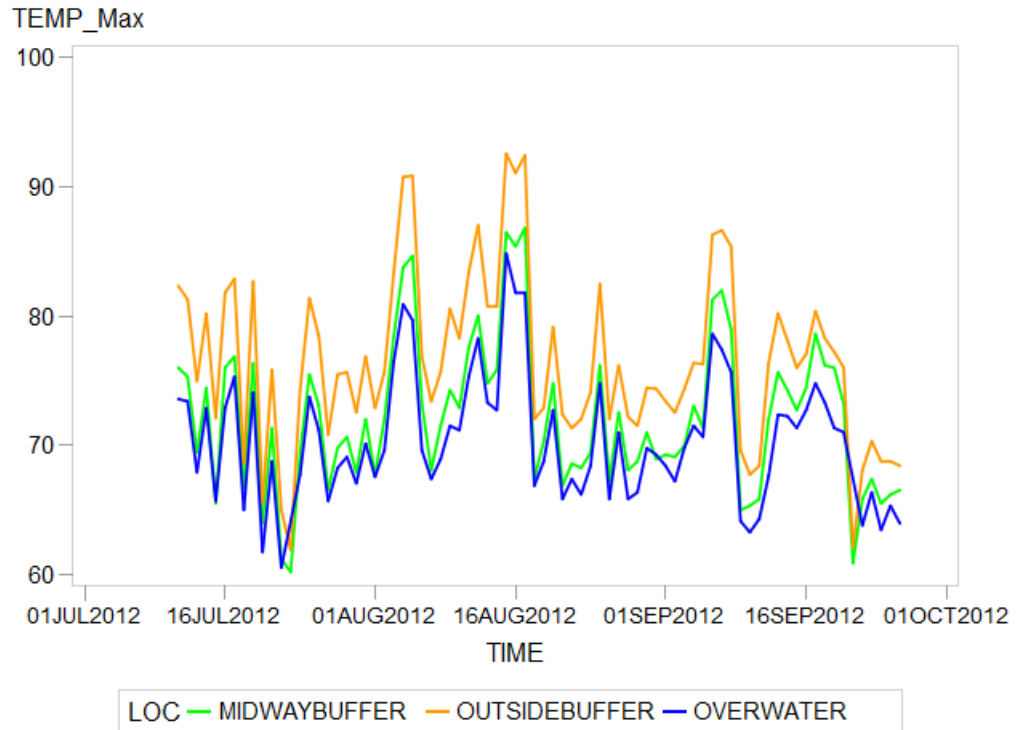
Appendix 15. Average Daily Maximum Temperature in 35' Buffer (North Bellingham Golf Course) by Sensor Location, 2012.
