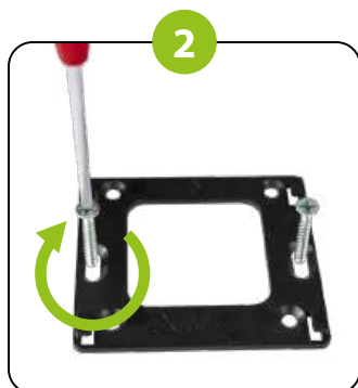
Screw the mounting plate to the box/wall
