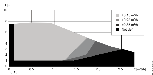
Accuracy of PWM feedback signal - flow estimation with water at 40 °C
