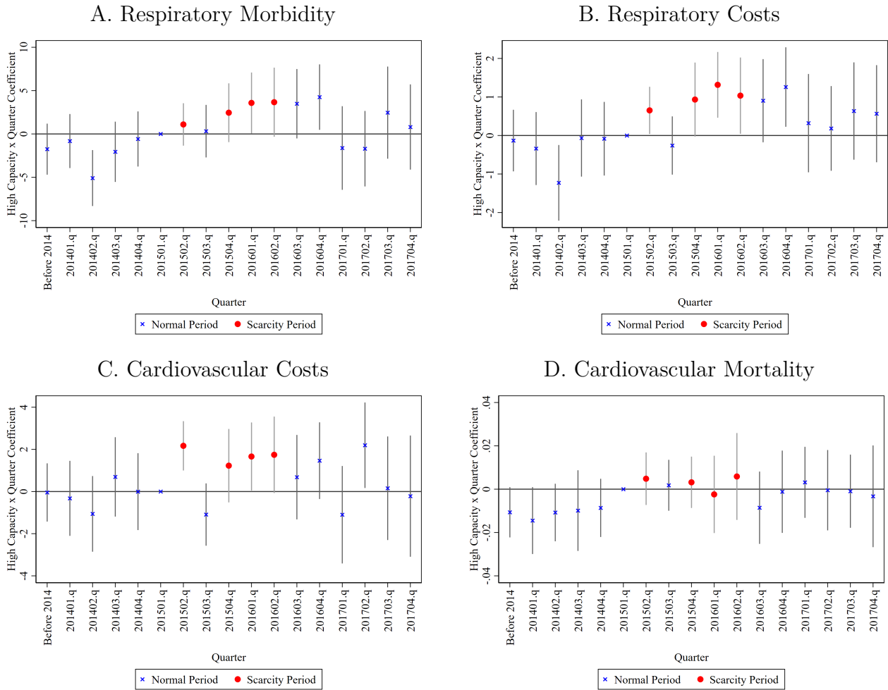
Figure A4: Event Study Results
