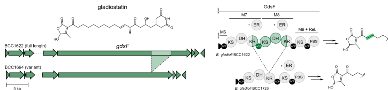
Figure 1: Structure and BGC of gladiostatins from B. gladioli . Catalytic domain level architecture of encoded protein showing intra-KR domain splice site and impact on compound structure.
