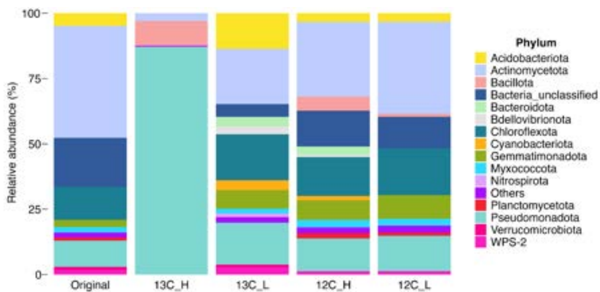
Figure 1: SIP: total microbial community. 13C_H: ^{13}\text{C} heavy fractions; 13C_L: ^{13}\text{C} light fractions; 12C_H: ^{12}\text{C} heavy fractions; 12C_L: ^{12}\text{C} light fractions.
