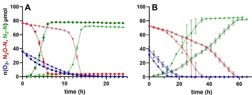
Figure 1: Consumption of added \text{N}_2\text{O} and \text{O}_2 and production of \text{N}_2 by vegetative or germinated Neobacillus vireti cells in pure culture (A) or soil slurry microcosm (B) experiments at 20°C. A, the cultures were inoculated with 5 \times 10^7 cells (circles) or spores (diamonds), the latter resulting in delayed \text{N}_2\text{O} consumption, due to germination, with a time lag of about 7 to 8 hours. B, soil microcosm experiments with (closed diamonds) or without (open diamonds) addition of N. vireti spores. The addition of spores resulted in an improved \text{N}_2\text{O} consumption rate. All values refer to \mu\text{mol} per vial (50 ml medium or slurry in 120 ml flasks) and were determined by gas chromatography using headspace samples.
