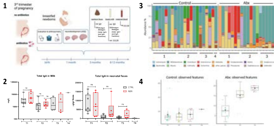
Figure 1: study design. Figure 2: Concentration of IgA in breast milk and neonatal feces. Figure 3: bacterial genera in neonatal feces. Figure 4: fecal microbiota diversity (observed features)
