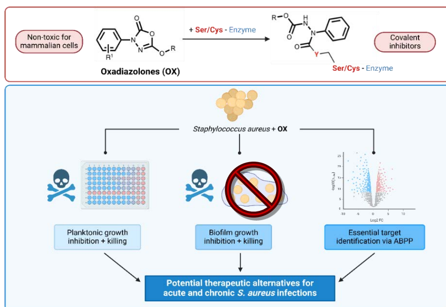
Figure 1: Oxadiazolone-core compounds inhibit and kill planktonic and biofilm-associated S. aureus through covalent inhibition of (Ser/Cys)-based enzymes, making them promising therapeutic antibacterial agents.
