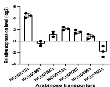
Fig. 1: Quantitative RT-PCR of arabinose transporters in lat-1 KO.
