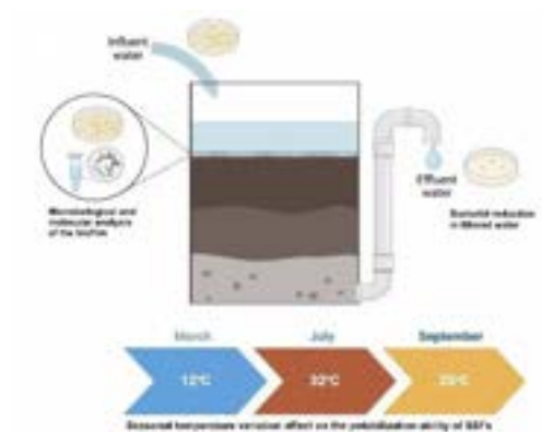
Figure 1: Experimental design of the study highlighting the three seasonal temperatures considered and their effect on both the microbial community in the biofilm and the potabilization efficiency of the slow sand filters.
