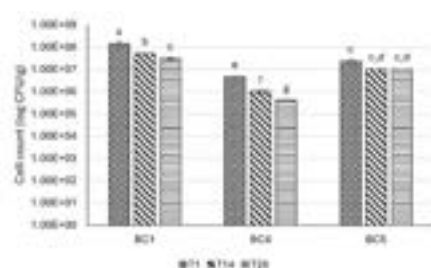
Figure 1: Cell load viability (log CFU/g) of the vaginal strains ( L. crispatus BC1, BC4 and BC5) in fermented milk during the storage in refrigerated conditions (after 1, 14 and 28 days from production).
