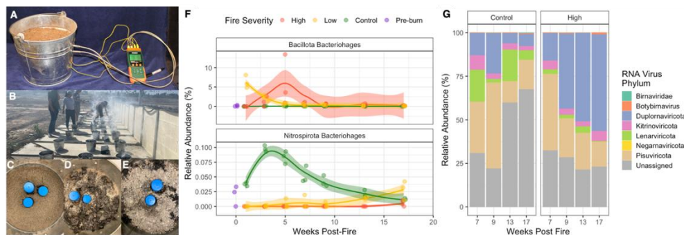
Figure 1: (A) Pyrocossm setup (adapted from Bruns et al. 2020, PLoS One), (B) simulated wildfire and (C-E) pyrocossm sampling. (F) Temporal changes in relative abundances of bacteriophages predicted to infect Bacillota (potential spore formers/ denitrifiers) and Nitrospirota (potential nitrifiers). (G) Changes in relative abundance of RNA viral phyla 7-17 weeks post-fire.
