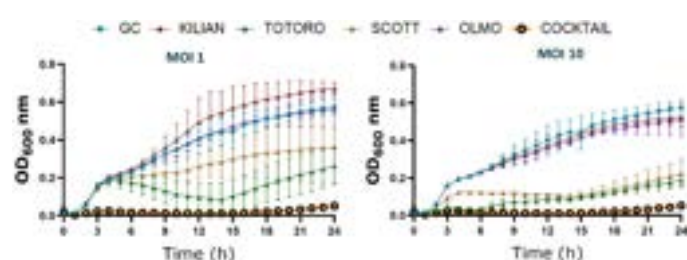
Figure 1: Optical density at 600nm measurements of K. pneumoniae - KPC clinical isolates tKp30 treated with single phages and phage cocktail composed of these phages at MOI 1 and 10. GC=growth control. Multiple unpaired Student's t-test were performed * p \leq 0.05 , The phage cocktail significantly controls bacterial load up to 24 hours at both MOI 1 and MOI 10, showing better performance compared to single phages: Only phages Kilian and Totoro are able to control bacterial growth at MOI 10 up to 6 hours. N=4.
