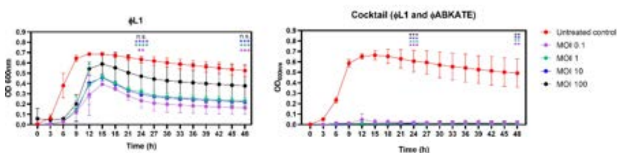
Figure 1: Growth kinetics of a XDR A. baumannii treated with: (A) phage L1. (B) phage cocktail composed of L1 and ABKATE phages. Multiple t -test between untreated control and each condition. p -value>0.05 n.s., p -value≤0.01 **, p -value≤0.001 ***, p -value≤0.0001 ****.
