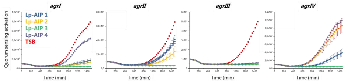
Figure 1: Lactiplantibacilli AIP structure impact its ability to interfere with S. aureus quorum sensing system. The activity is assessed by QS-regulated expression of Yellow Fluorescent Protein (YFP) in P3- yfp reporter systems in the four- agr -allelic groups measured as YFP accumulation overtime.
