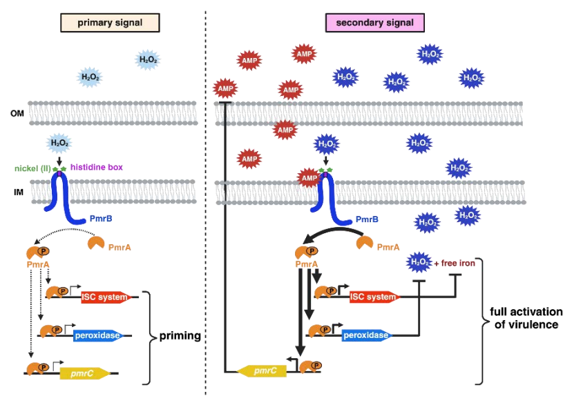
Summary Figure: Model for the priming effect by H_2O_2 under control of the PmrA/PmrB system in A. baumannii . (Left panel) During infection, bacteria usually
