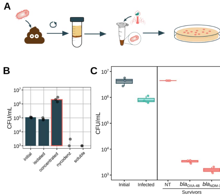
Figure 1: A-B) We can isolate and concentrate microbiota fecal samples to make the cells more accessible for infection. C) No killing effect is observed when using a non-targeting phagemid (NT). Treatment of fecal samples colonized by bla NDM-1 and bla OXA-48 producing Enterobacteriaceae with the phagemid (multiplicity-of-infection = 10^3 ) resulted in the elimination of more than 99.98% of the target resistance genes.
