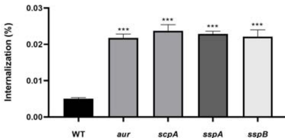
Figure 1: Invasive behavior of S. aureus USA300 WT and the aur , scpA , sspA or sspB mutant strains towards human lung epithelial cells. The numbers of internalized WT or single protease mutant bacteria were determined after 1 h of infection and 30 min incubation with lysostaphin. To this end, the cells were lysed with 0.05% SDS and the released bacteria were collected and counted by plating on TSA plates. The internalization of the WT and mutant bacteria is presented as the proportion of the total bacterial count used for the infection. The bar plot shows the mean values from three individual experiments and the error bars show the respective standard deviation. Statistical significance was assessed by two-tailed t-tests. A P-value < 0.05 was considered significant (***, p < 0.005 ).
