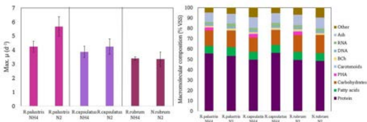
Figure 1: Growth rates (left) and macromolecular composition (right) of three PPB strains ( Rp.s palustris , Rb. capsulatus , and Rp. rubrum ) under photoheterotrophic conditions using NH_4^+ (reactive nitrogen) or N_2 (diazotrophic). Error bars represent the standard error.
