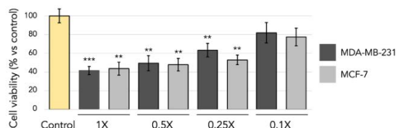
Figure 1: Cell viability of MDA-MB-231 and MCF- 7 cell lines after 24 hours of contact with bacterial secretomes from consortium 7: MTT test with different secretome concentrations (1X, 0.5X, 0.25X and 0.1X). Significant differences are indicated by * ( p<0.05 ), **( p<0.01 ), or *** ( p<0.001 ) in comparisons between the no-treatment control (yellow) and the trials with secretome treatment.
