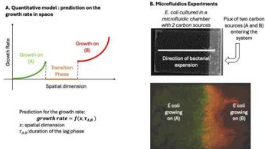
Figure 1: A –The mathematical model predicts a growth rate that depends on the concentrations of the nutrients, consequently it is a function of the spatial dimension and of the lag time needed to transition from nutrient (A) to (B). B - Microfluidics experiments where E. coli , engineered to express mCherry or GFP according to the carbon source consumed, grows in microfluidics chambers. There, bacteria consume two nutrients. The preferred nutrient (B) is consumed in proximity of the opening of the chamber, until is depleted, while bacteria at the back grow on the second nutrient (A), pushing bacteria in front of them out of the chamber, and entering in regions where the first nutrient is still present, this induces a transition from carbon source (A) to (B).
