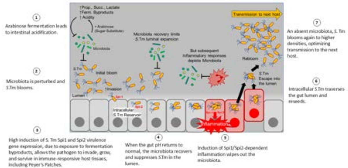
Summary Figure. Ingestion of arabinose promotes gut colonization and virulence in Salmonella Typhimurium .
