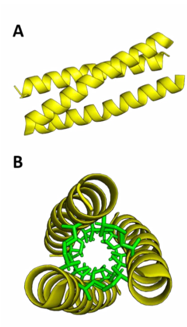
Figure 1: side view (A) and top view (B) of the GCN4-pII trimer bundle.
