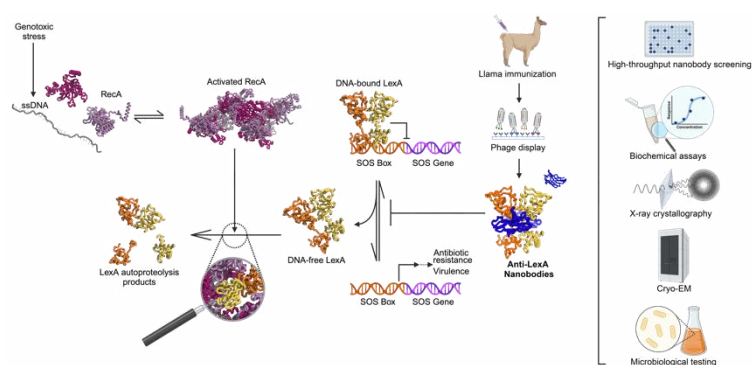
Figure 1: Overview of work. Mechanistic elucidation and nanobody-based suppression of the response were investigated by structural, biophysical, biochemical and microbiological techniques.
