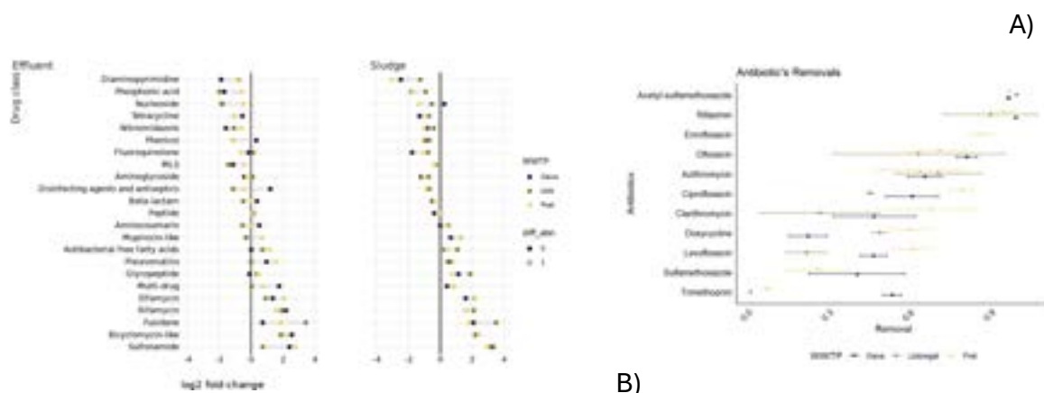
Figure 1: A) Removal efficiency of ARGs by target drug in the Gava, Llobregat and Prat WWTPs. Negative fold-change, removal; positive-fold change, enrichment. B) Antibiotic removal by antibiotic family in the Gava, Llobregat and Prat WWTPs.
