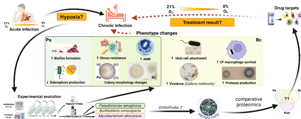
Figure 1: Graphical abstract showcasing our methods and key results , including a developed tool for orthology comparisons of proteomic datasets; five proteins commonly altered by long-term hypoxia in Pa , Bc and Mab which are drug targets, common and distinct changes of phenotype in Pa and Bc , which lead to a conclusion that hypoxia contributes to chronic infection adaptation and may affect treatment efficiency.
