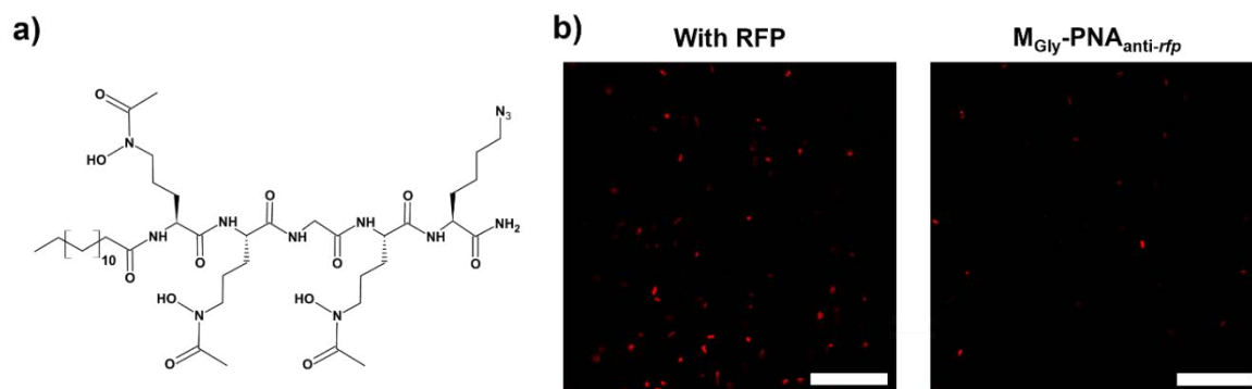
Figure 1: a) Structure of M Gly siderophore. b) Inhibition of rfp gene expression by M Gly -PNA anti-rfp conjugate, shown as decreased fluorescence intensity, compared to untreated E. coli \Delta fur RFP bacteria. Scale bar: 20 \mu m.
