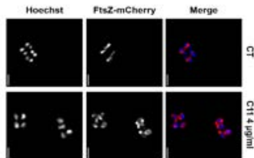
Figure 1: Fluorescence microscopy images of S. aureus TD276 carrying the FtsZ-mCherry.
