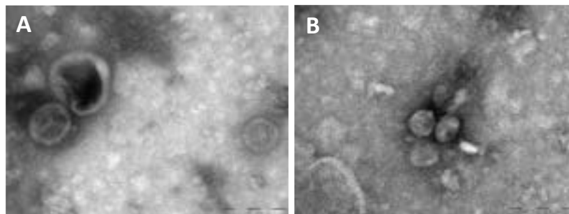
Figure 1: TEM images (negative staining) of extracellular OMVs of KpB199 (A) and KpB10 (B). (Scale bar- 100 nm; 300 X magnification).
