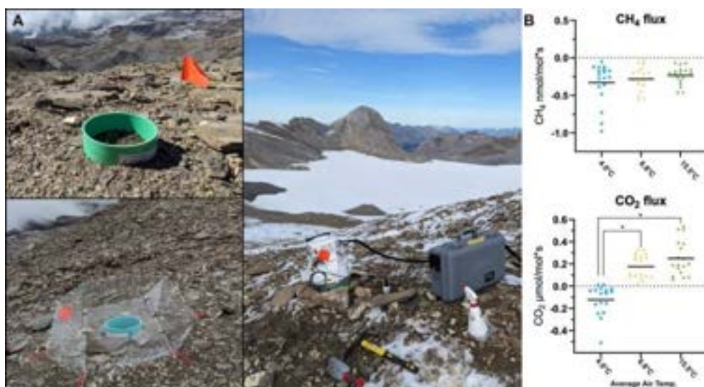
Figure 1: A) Example of experimental warming plots and GHG flux measurements in high-altitude permafrost affected sites. B) \text{CO}_2 and \text{CH}_4 fluxes across three fall days.
