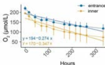
Figure 1 | Gene Abundance and Activity in Sea Cave Environments. (A) Average gene copy numbers per organism for photosynthesis marker genes ( psaA and psbA ). (B) Average gene copy numbers per organism for chemosynthesis marker genes ( cooS , coxL , NiFe G1 and G2 , amoA , nxrA , fcc , sqr , and soxB ). (C) Comparison of ^{14}\text{CO}_2 incorporation rates between entrance and inner sea cave sediments supplemented with different energy sources. (D) Oxygen consumption rates in sea cave entrance and inner sediments.
