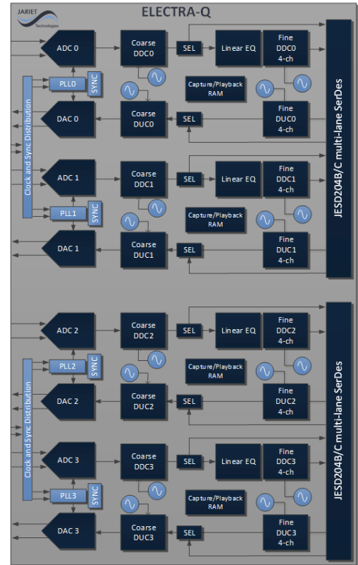
Electra-Q Block Diagram
