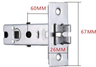
A1 Lock Body (center distance 60 mm)
