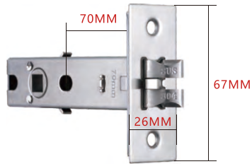
A2 Lock Body (center distance 70 mm)
